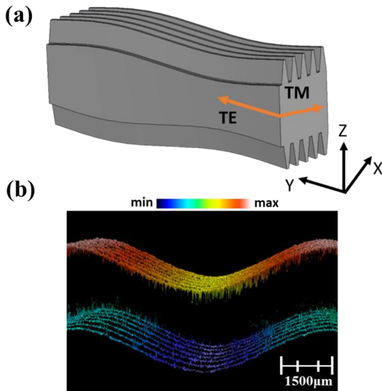
Fig.9. Schematic representation of Sinusoidal silicon-based high contrast grating; (a) 3D representation of a developed grating (b) profile of a fabricated grating along YZ-axis.
