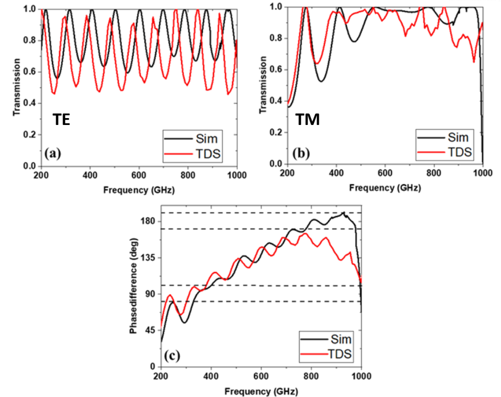
Fig.8. Double-sided dielectric-based high contrast grating (a) Transmission spectra of TE polarization, (b) TM polarization and (c) Phase retardation for simulation (Black) and measurements (Red).
